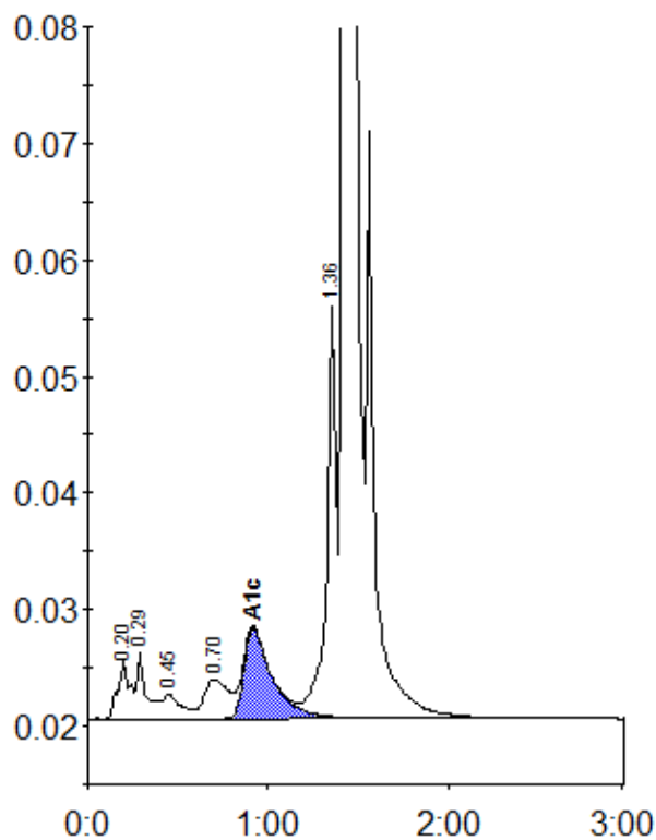
Peak table - ID: 10425119
